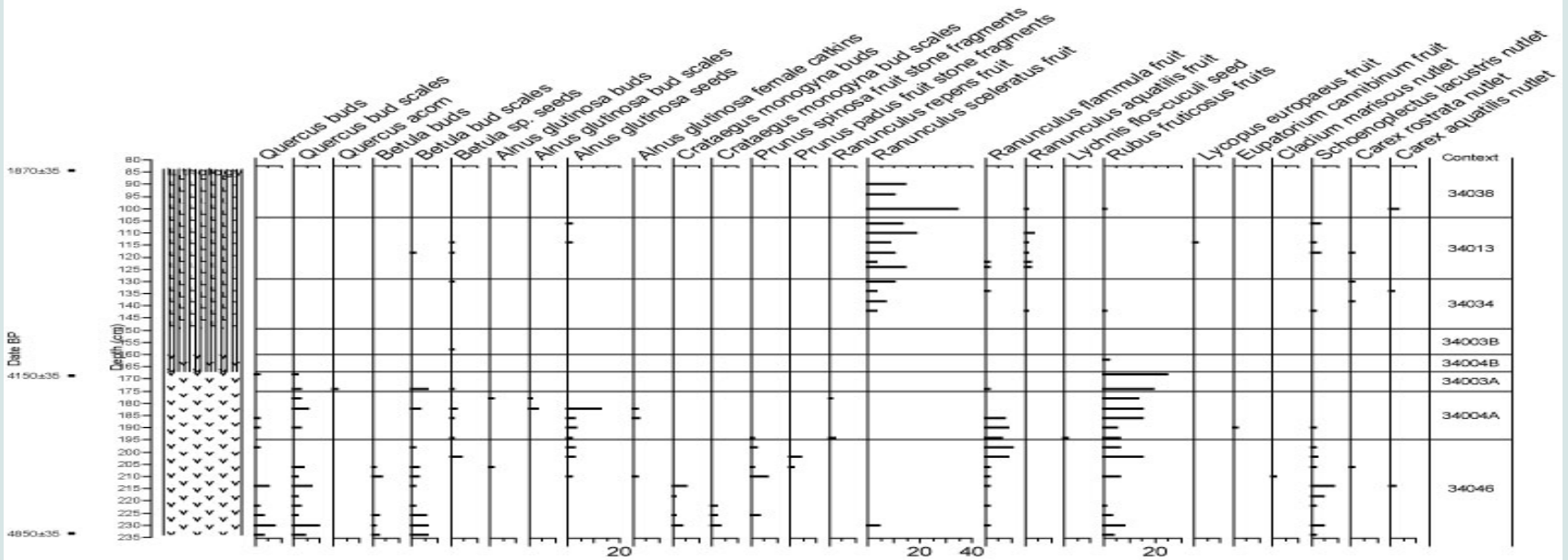
NWB-03 Monolith 1 Selected Plant Macrofossil Diagram
